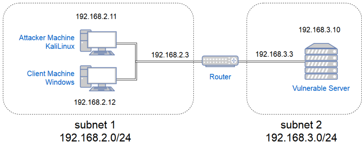
Figure 1 Lab Setup
